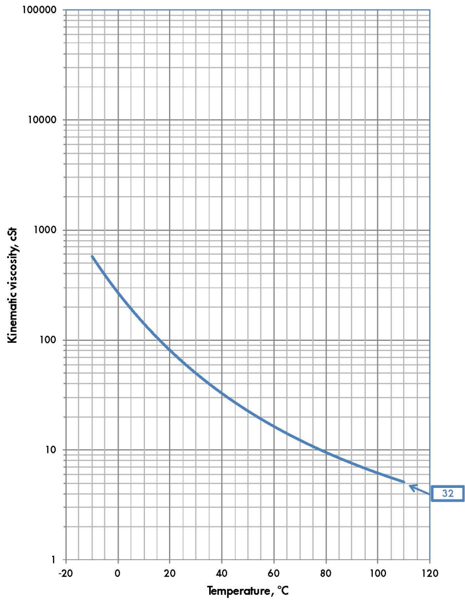
Viscosity - Temperature Diagram Shell Corena S2 RJ
